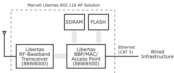
Fig 2. Libertas WLAN 802.11b Access Point Chipset (88W8000 and 88W8500) Applications Diagram
