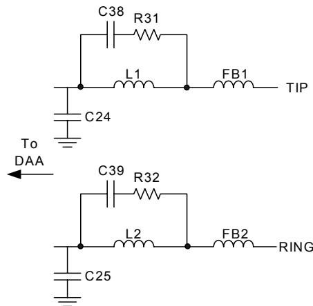
Figure 35. Notch Filter for CISPR22 Compliance
