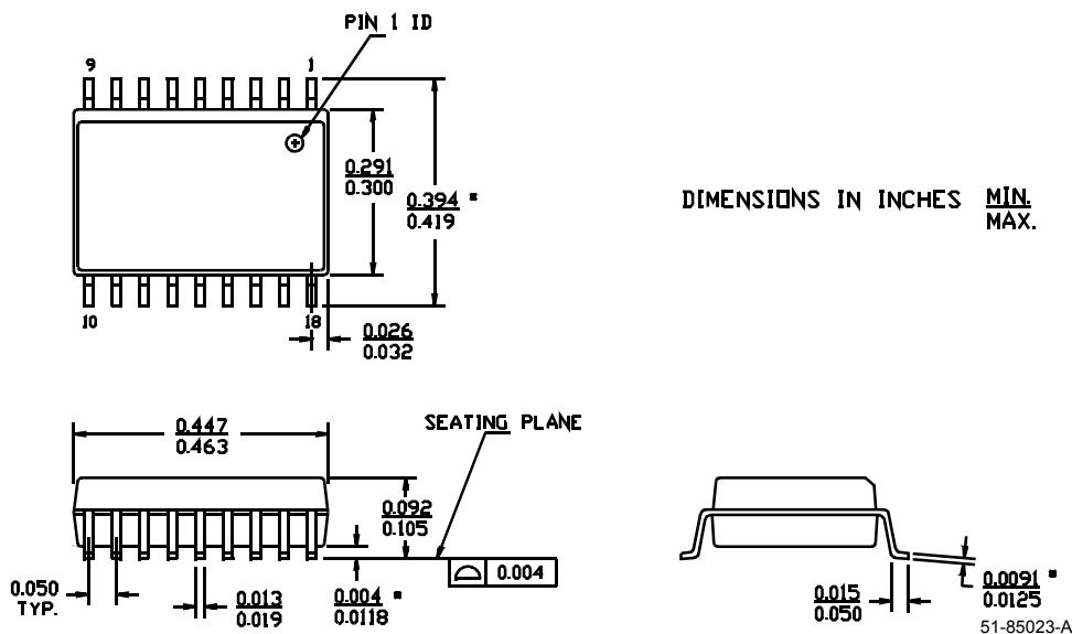
18-Lead (300-Mil) Molded SOIC S3
