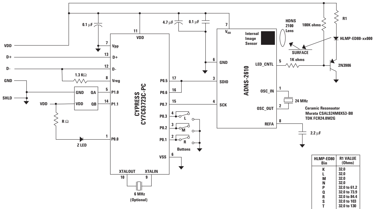
Figure 8. Circuit block diagram for a typical corded optical mouse using an Avago ADNS-2610 optical mouse sensor.
