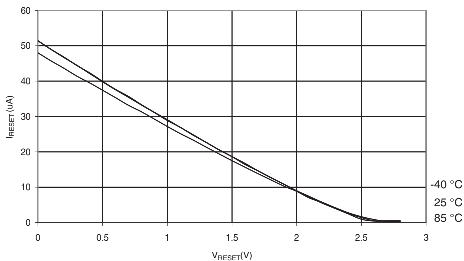
Figure 28-20. Reset Pull-up Resistor Current vs. Reset Pin Voltage ( V_{CC} = 2.7V )
