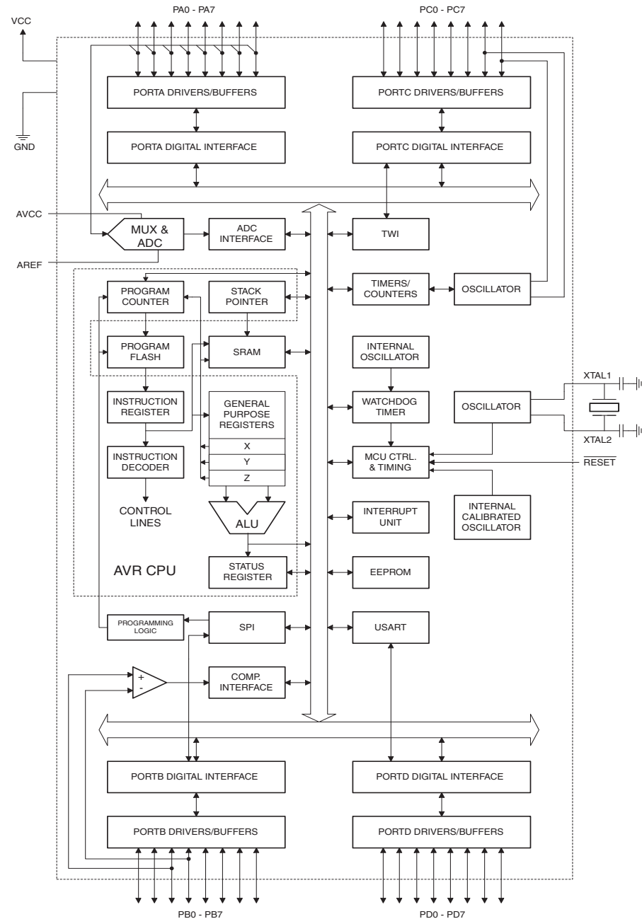
Figure 2-1. Block Diagram
