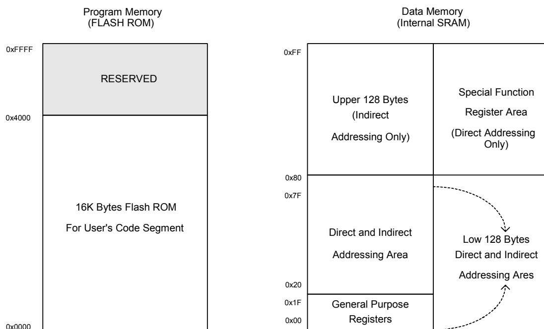
Figure 1-1. SH68F83 Program/Data Memory Map
