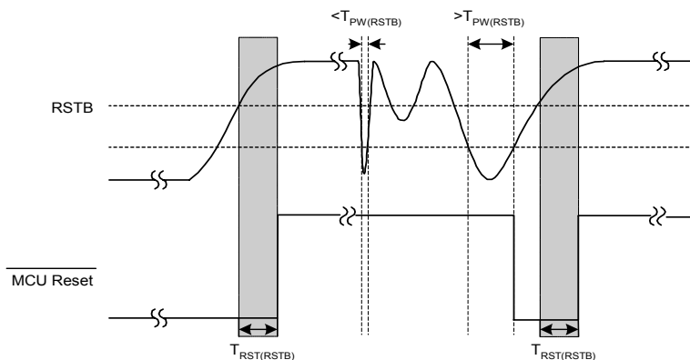
Figure 5-5. External Reset
