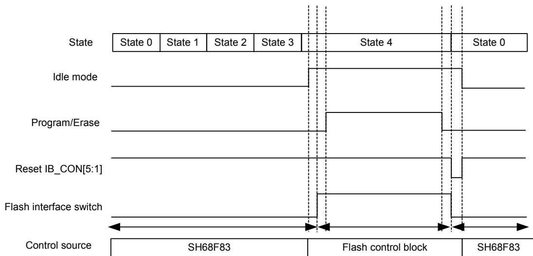
Figure 11-4. Flash Control Timing Diagram
