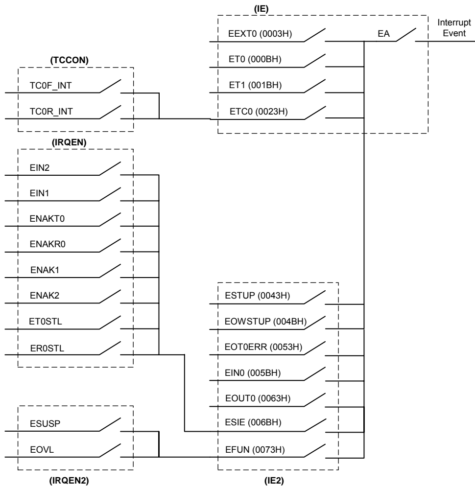
Figure 7-1. Interrupt Structure
