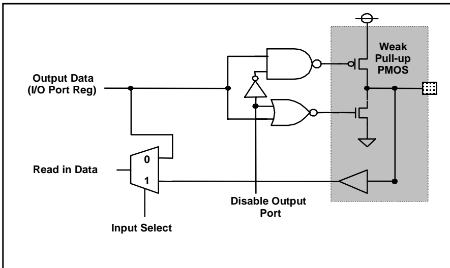
Figure 6-1. PORT Configuration-1
