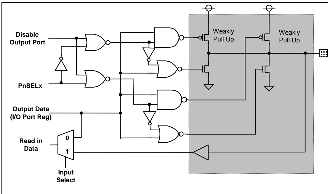
Figure 6-2. PORT Configuration-2
