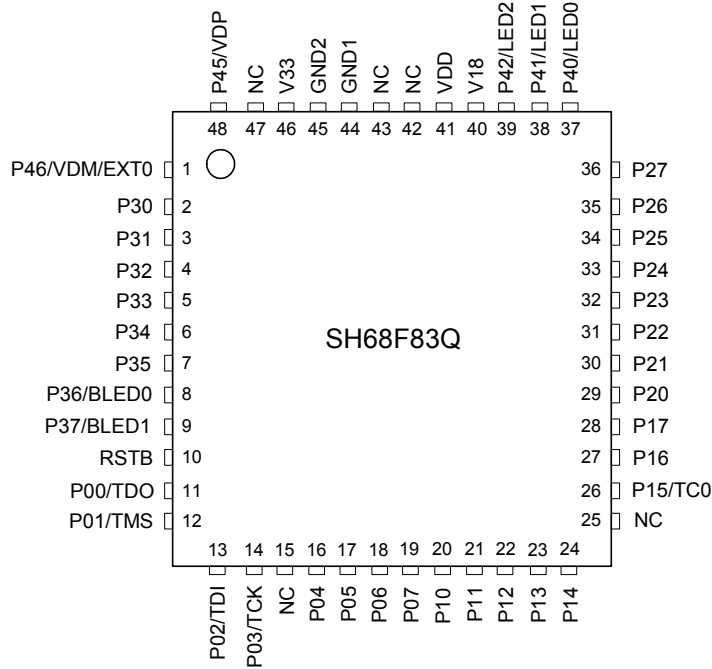
SH68F83 48-Pin (QFN) Package
